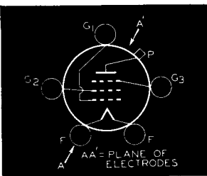
Bottom View of 804 Socket Connections
