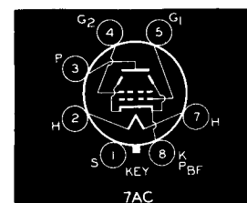
Bottom View of 1614 Socket Connections
