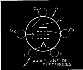
Bottom View of 803 Socket Connections
