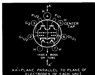
Bottom View of 829 and 832 Socket Connections
