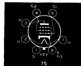
Bottom View of 1613 Socket Connections
