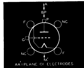
Bottom View of 810 and 1627 Socket Connections
