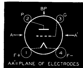
Bottom View of 1608 Socket Connections
