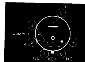
Bottom View of VR-75, 105, and 150 Socket Connections
