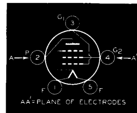
Bottom View of 1610 Socket Connections
