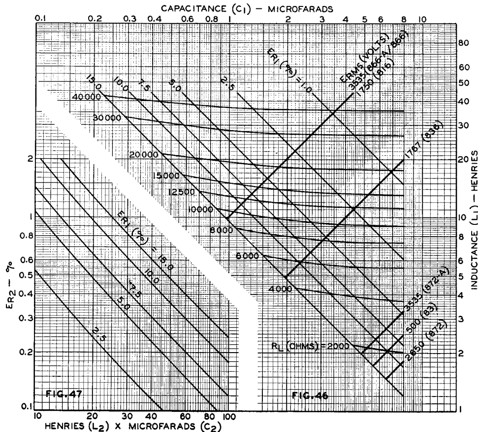
Fig. 46—Curves for choice of filter values for (1) the first section of a double-section filter, or (2) a single-section filter.
