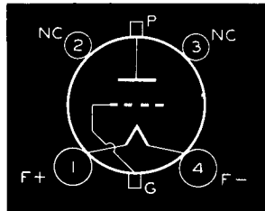
Tube Mounting Position VERTICAL—Base up or down HORIZONTAL—Not recommended
