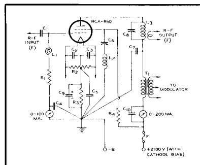
PLATE-MODULATED TETRODE R-F AMPLIFIER Power Output 100 Watts (Approx.)
